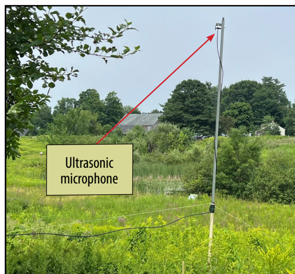
Figure 3. Photo of deployment set up at Gilsland Farm.
