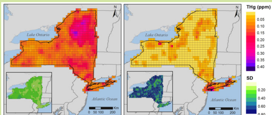
Spatial distributions of average tissue total mercury concentrations in parts per million in aquatic (left) and terrestrial (right) biota across New York State from 1969 — 2017.
